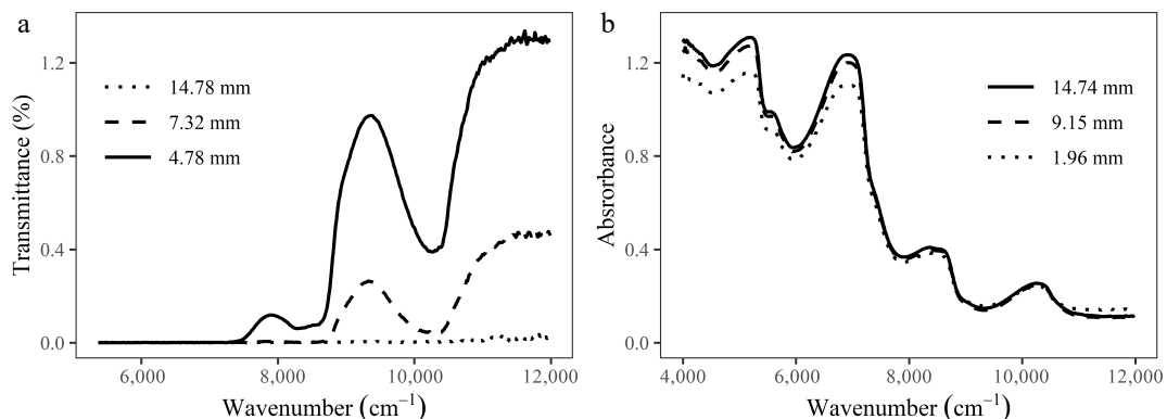
Fig. 2 (a) Typical transmission and (b) reflectance spectra for an avocado at varying thicknesses.
