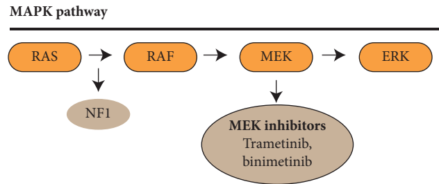
FIGURE 3: Schematic diagram of MAPK [74].
