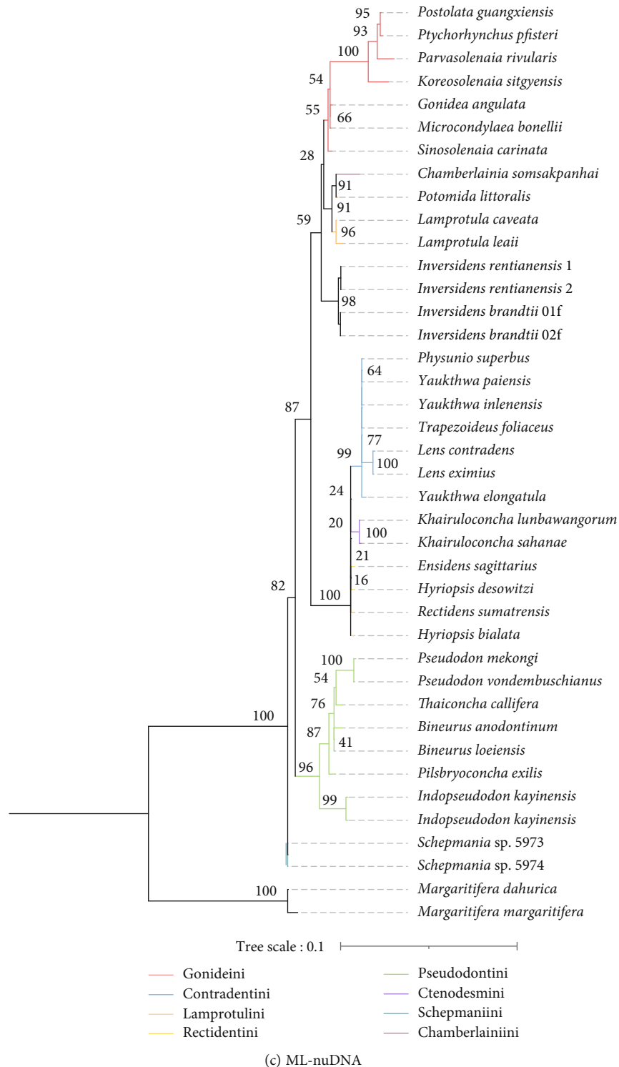
FIGURE 5: Phylogenetic trees inferred from Bayesian inference (BI) and maximum likelihood (ML) analyses. (a) Phylogram of BI and ML tree based on the mtDNA gene dataset (COI+ND1+16S rRNA). Numbers at nodes are support values for ML (bootstrap support (BS))/BI (posterior probability (PP)). (b) Phylogram of BI tree based on the nuDNA gene dataset (18S rRNA+28S rRNA). Numbers close to the nodes indicate for PP values. (c) Phylogram of ML tree based on nuDNA gene dataset (18S rRNA+28S rRNA). Numbers close to the nodes indicate BS values. Both Inversidens species are shown in red font. Colored clades represent eight tribes of the subfamily Gonideinae.
