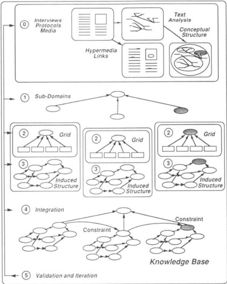
Figure 33 Integration of knowledge acquisition techniques
