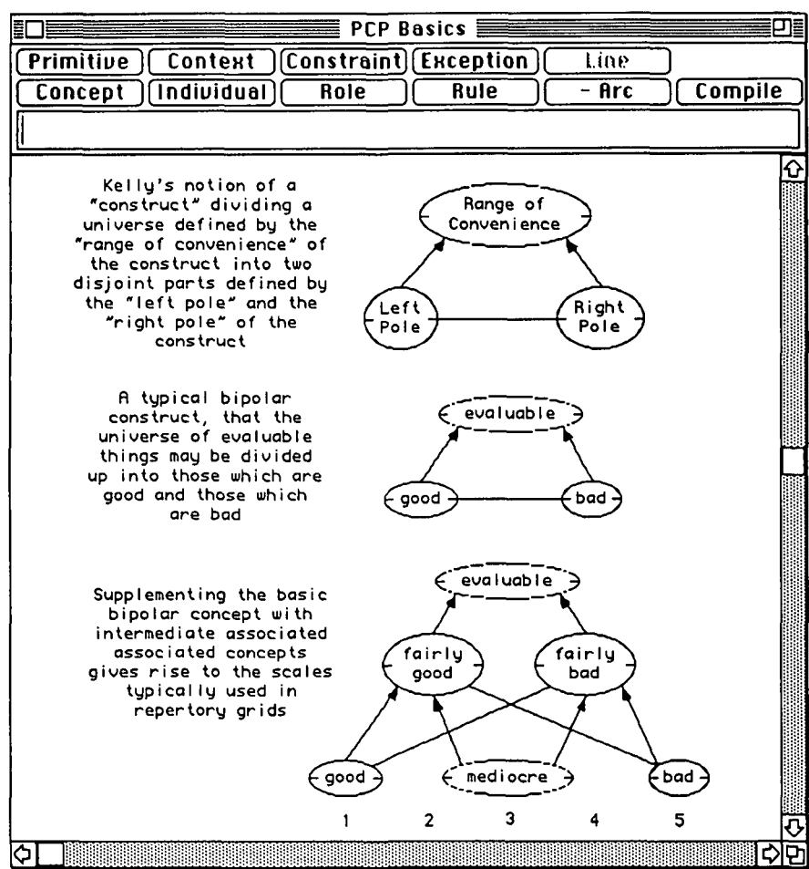
Figure 2 Representation of abstract and specific constructs and scales in a visual language for specifying definitions and assertions in the intensional logic
