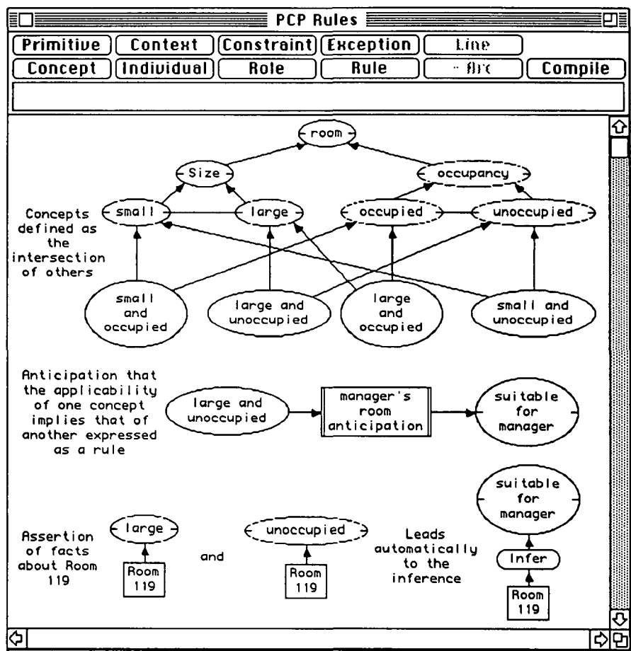
Figure 3 Concepts defined in terms of others, and their application to representing anticipations as rules supporting inference
