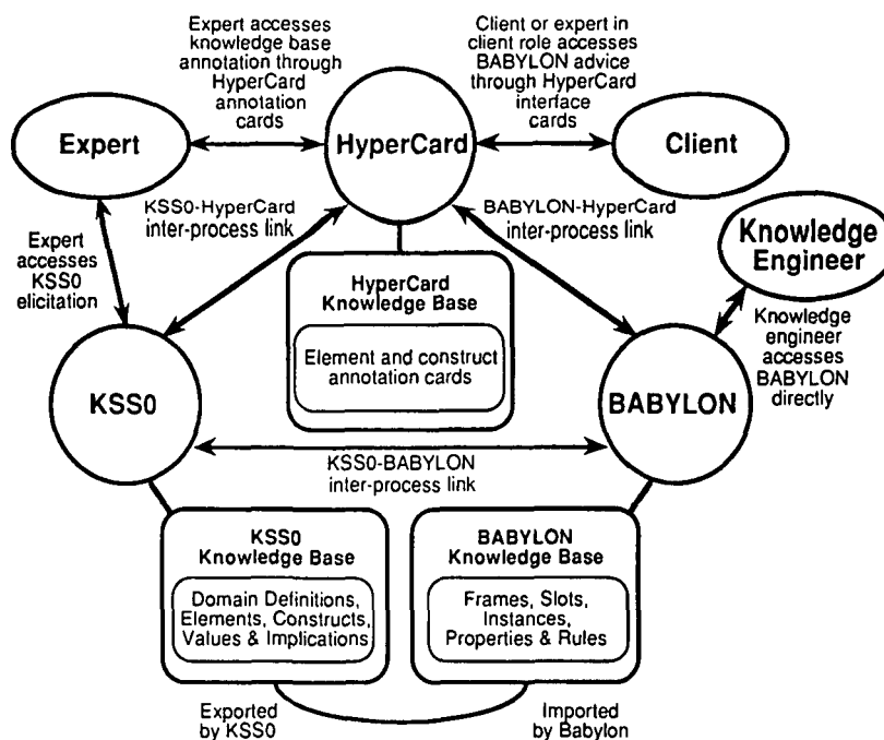
Figure 31 Integration of hypermedia, knowledge acquisition and expert system shell
