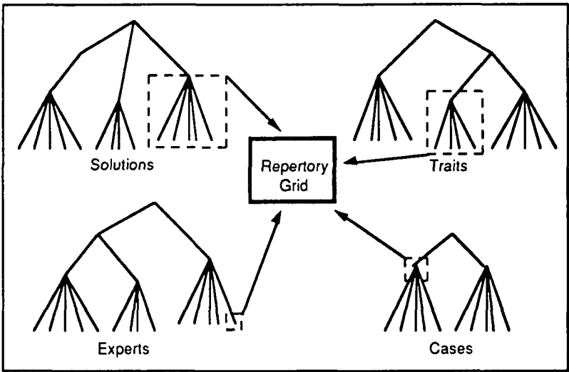
Figure 24 AQUINAS extended repertory grid structure (Boose & Bradshaw, 1987)
