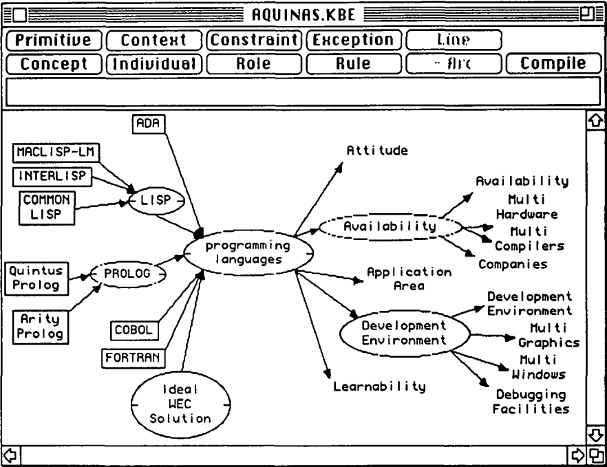
Figure 29 AQUINAS language advisor solution and trait hierarchies in the grapher
