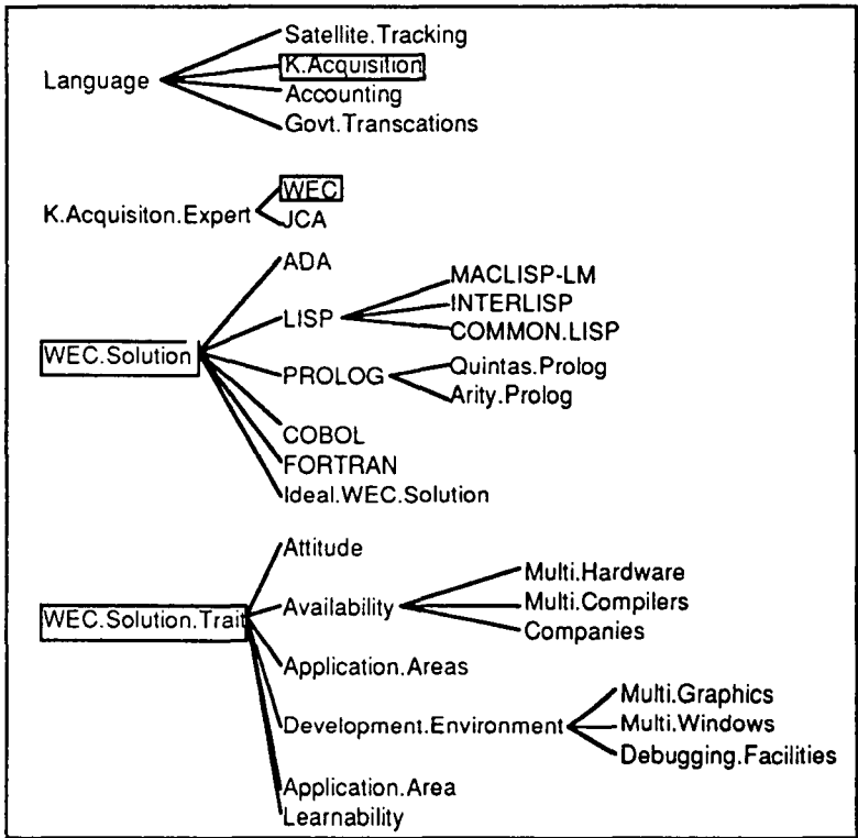
Figure 25 Programming language advisor hierarchies in AQUINAS (Boose & Bradshaw, 1987)
