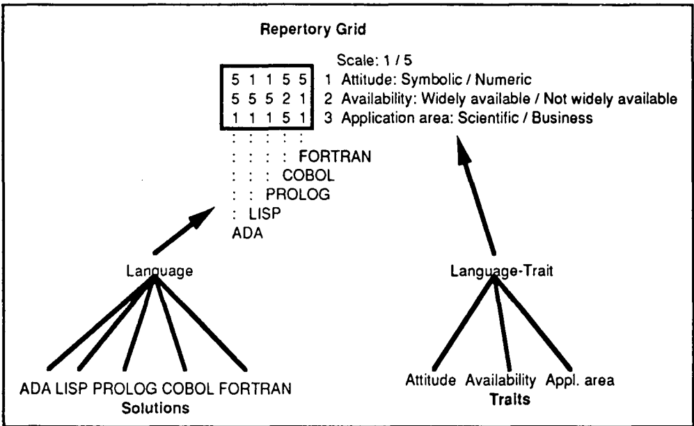
Figure 26 Defining a grid from a hierarchy in AQUINAS (Boose & Bradshaw, 1987)
