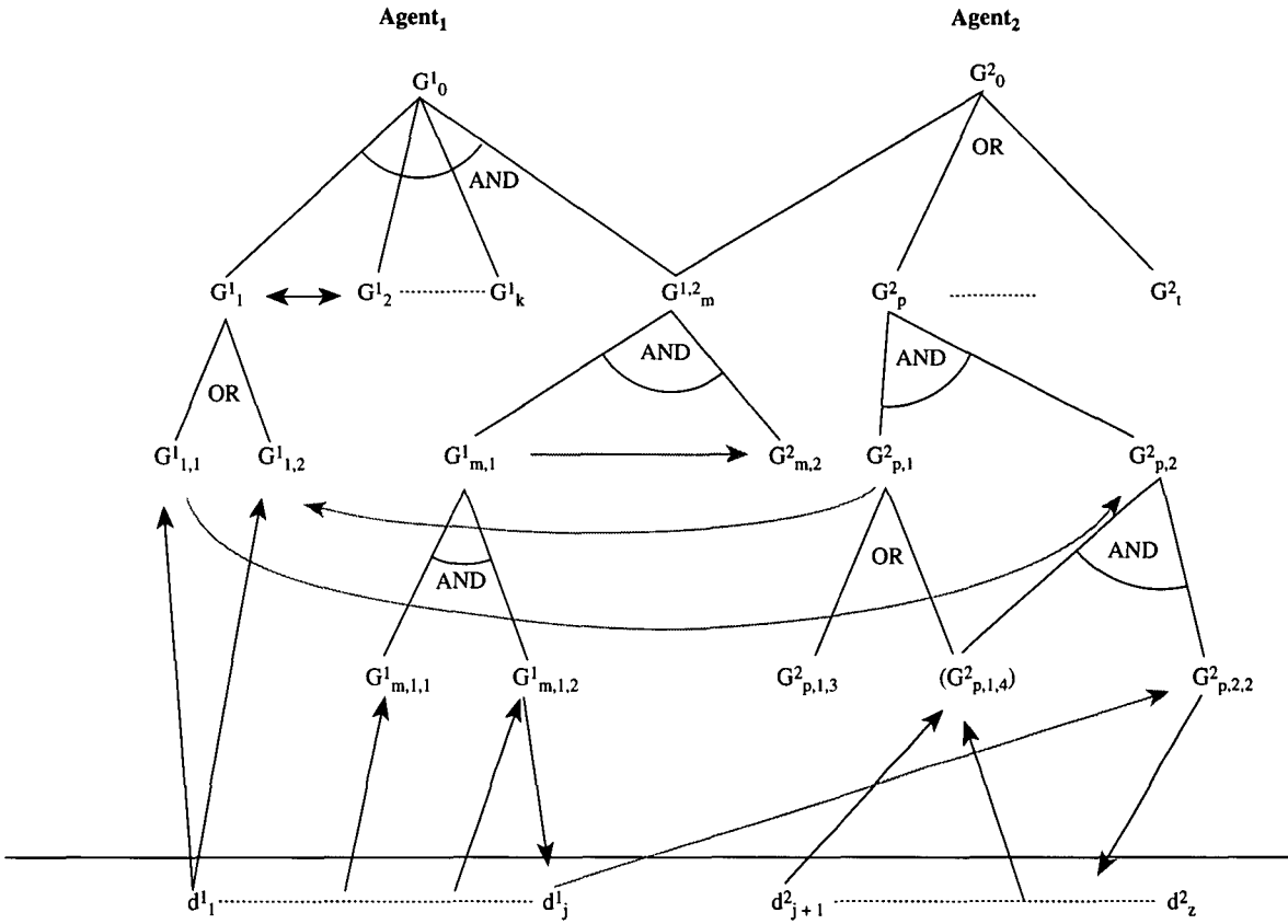
Figure 2 A distributed goal search tree involving Agent 1 and Agent 2 . The dotted arrows indicate interdependencies between goals and data in different agents, solid arrows dependencies within an agent. Superscripts associated with goals and data indicate the agent which contains them
