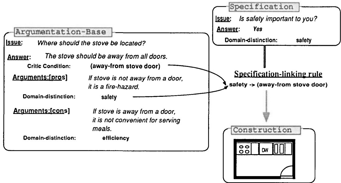
Figure 6 Derivation of the Specification-Linking rules. The domain distinction associated with a specification item is paired with a matching pro or con argument in the hypermedia issue base. The critic condition associated with an answer is linked with the domain distinction to form a specific critic rule.
