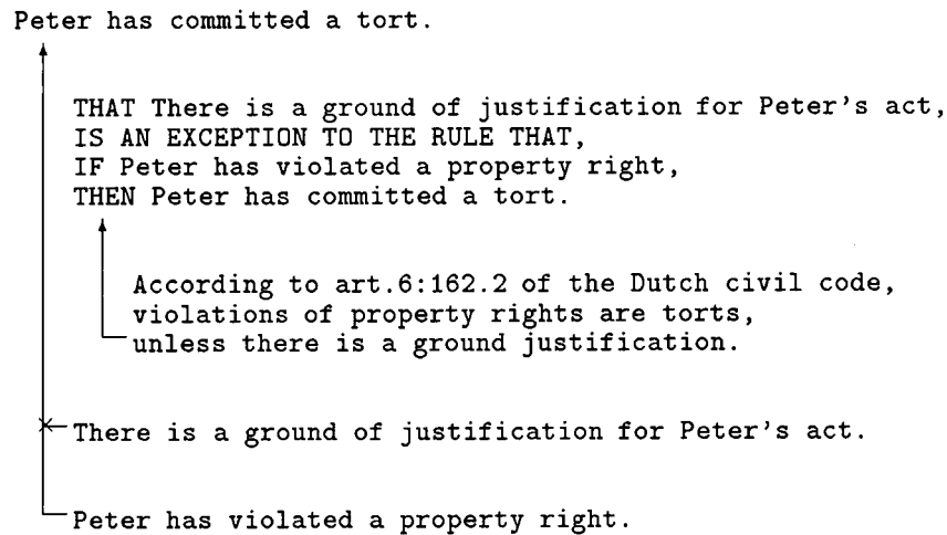
Figure 4 An argument structure represented in the ArguMed System (Verheij, 1999). The conclusion Peter has committed a tort that is derived from the fact Peter has violated a property right has the warrant IF Peter has violated a property right, THEN Peter has committed a tort with backing According to art.6:162.2 of the Dutch civil code, violations of property rights are torts, unless there is a ground justification. In addition, there is the undercutter There is a ground of justification for Peter's act obtained by the exception to the warrant.
