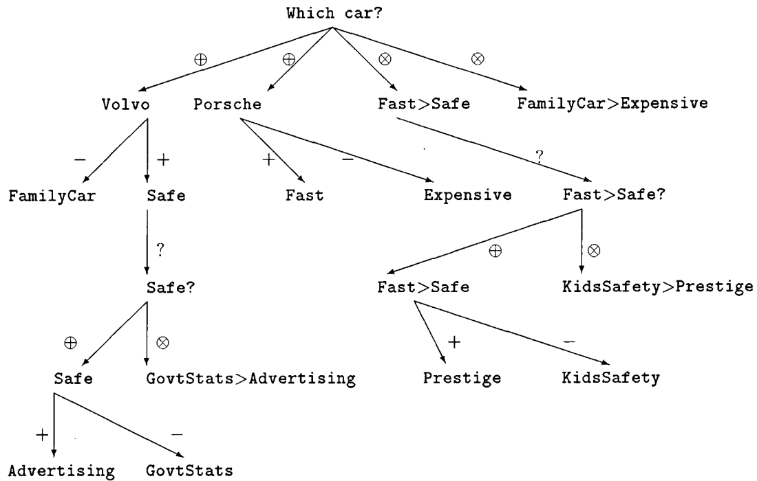
Figure 5 An example of a Zeno argumentation graph where ? denotes an issue, + denotes a pro, - denotes a con, \oplus denotes a choice, and \otimes denotes a constraint. In this example, the main issue is which car?. There are two choices Volvo and Porsche and two constraints: Fast is preferred to Safe; and FamilyCar is preferred to Expensive. There are pros and cons for the choices. Of these pros and cons, the only issue is Safe?. The others are accepted as undisputed facts. The only choice for the issue Safe? is Safe and there is a pro and a con, both of which are accepted as undisputed facts. However, there is also a constraint that GovtStats (Government Statistics) are preferred to Advertising. In an analogous way, the constraint Fast is preferred to Safe is also an issue. This constraint can be rejected because the con KidsSafety is preferred to the pro Prestige. This example is adapted from Gordon & Karaçapilidis (1997).
