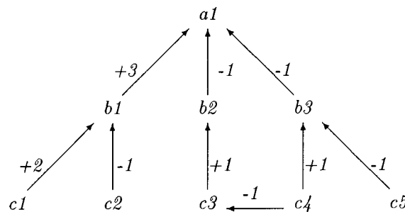
Figure 7 A Binary WeFA graph with the factor of interest being a1 . b1 has a direct positive influence on a1 , and b2 and b3 have direct negative influences on the aim. c1 , c4 and c5 have an indirect positive influence on a1 , and c2 , c3 and c4 have an indirect negative influence on a1 . As an example of a scenario, we could have c1 , c2 and c3 true. From this, we would get c4 and c5 false by default, and b1 , b2 , and b3 true by inference, and finally a1 true by inference.
