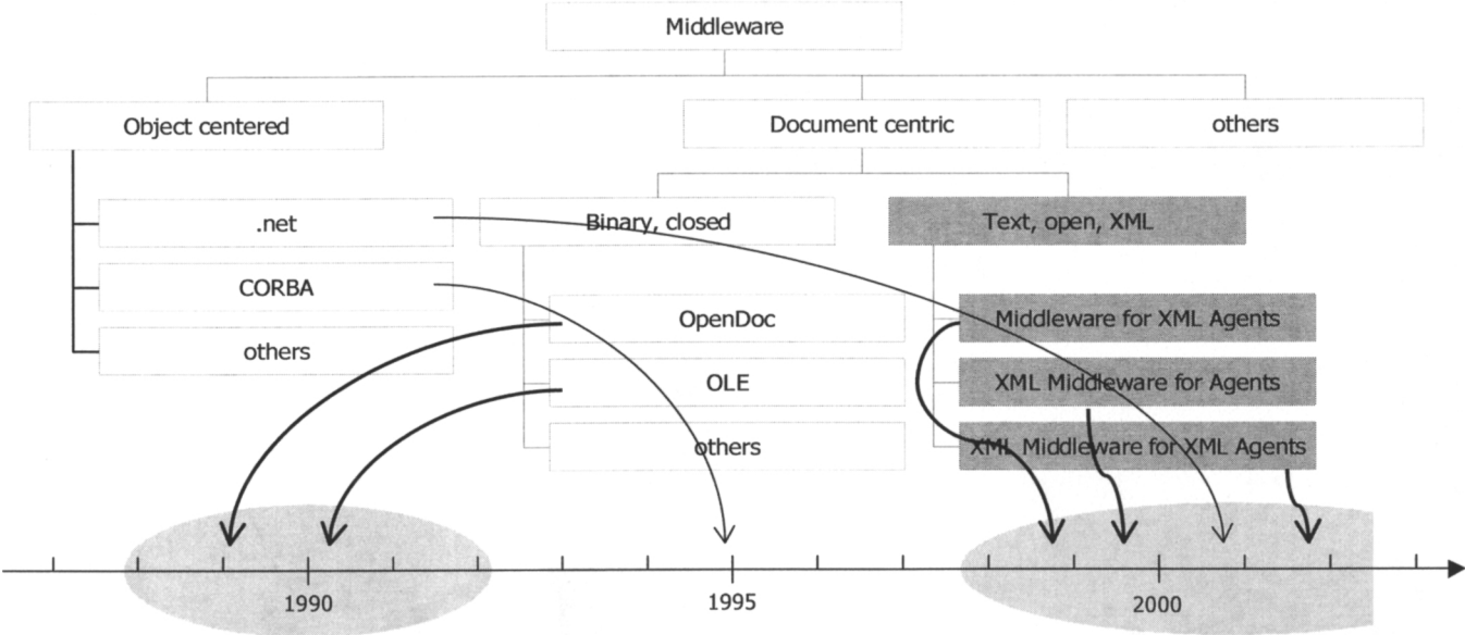
Figure 1 Document-centric middleware
