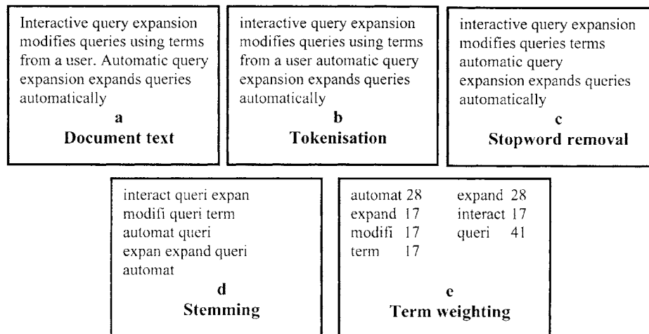
Figure 1 Indexing a document
