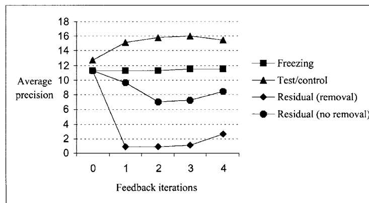
Figure 13 Average precision over 4 iterations of feedback
