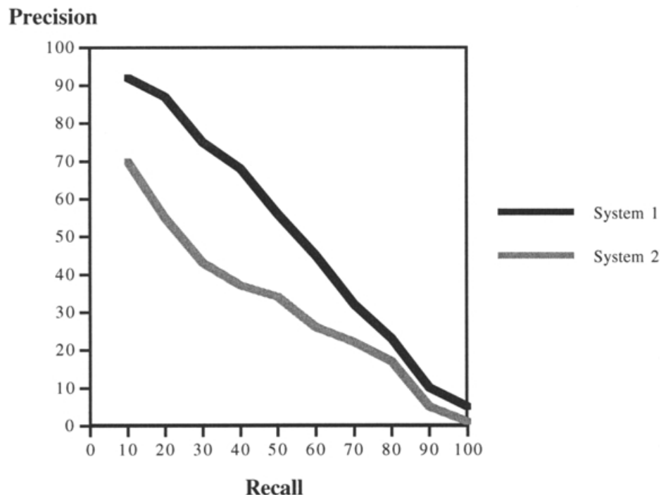
Figure 11 Example recall-precision graph
