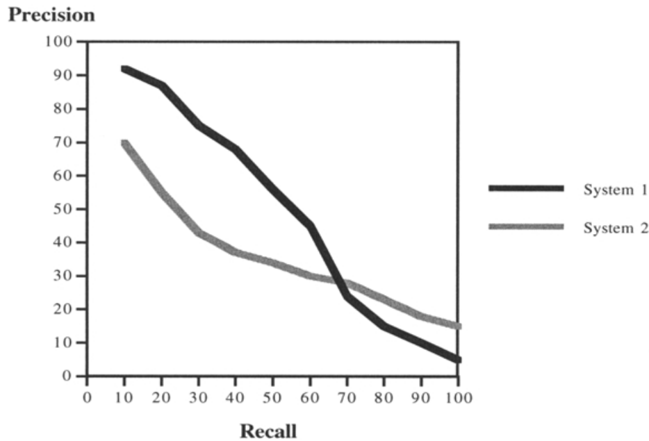
Figure 12 Example recall-precision graph
