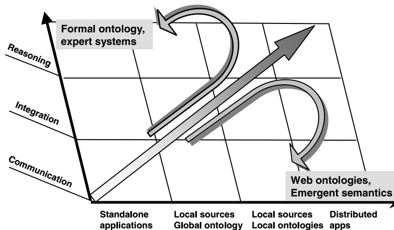
Figure 7 Complexity increases rapidly as we try to move along both axes at the same time due to the difficulty of maintaining formality in decentralized settings. The result is a bifurcation of technology development in two distinct directions
