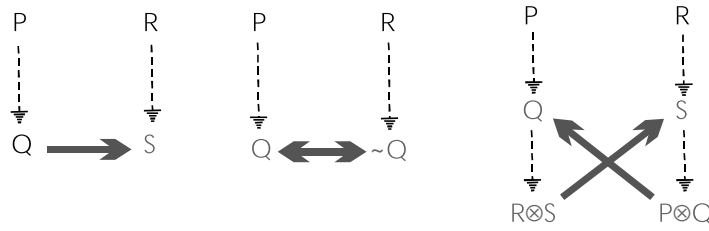
Figure 23 Pollock diagrams
