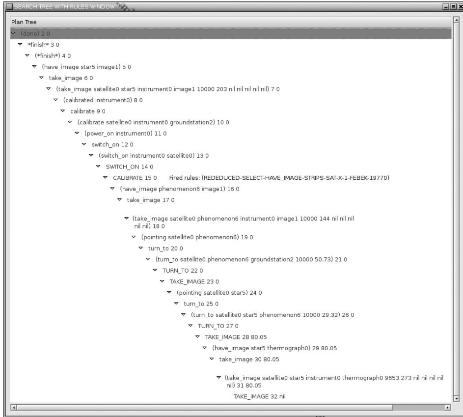
Figure 11 Search tree view
