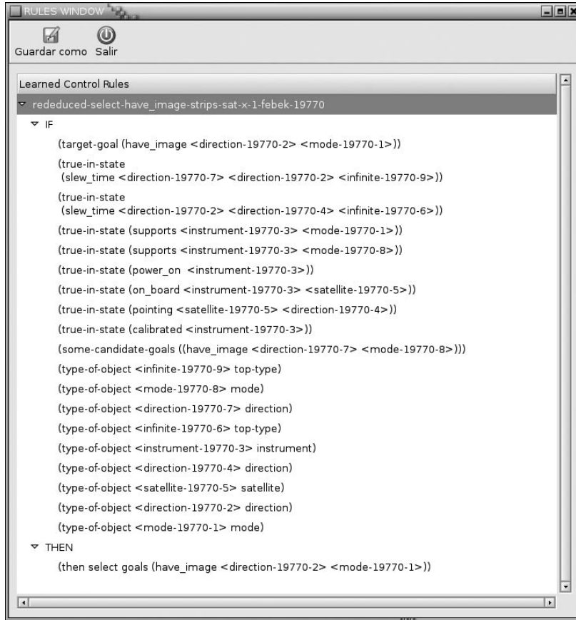
Figure 8 Automatically learned control rules for the satellite domain
