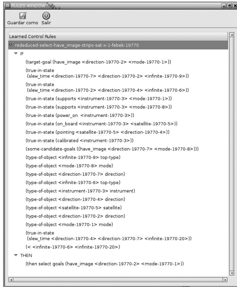
Figure 10 An example of user refined rule for the satellite domain
