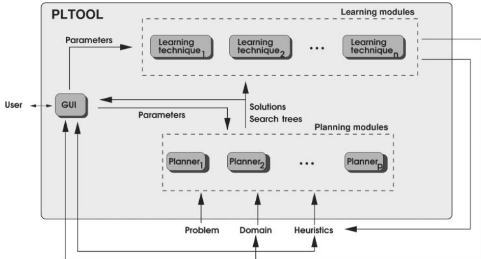
Figure 1 High-level architecture of PLTOOL
