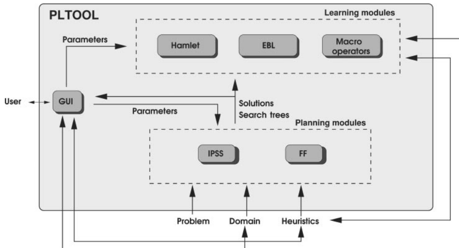
Figure 2 Current implementation of PLTOOL architecture
