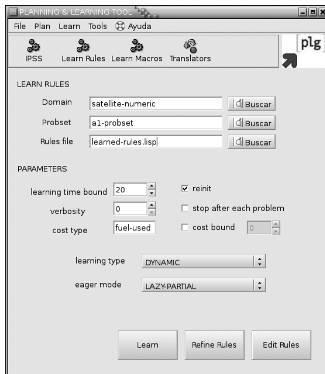
Figure 7 Learning window in PLTOOL
