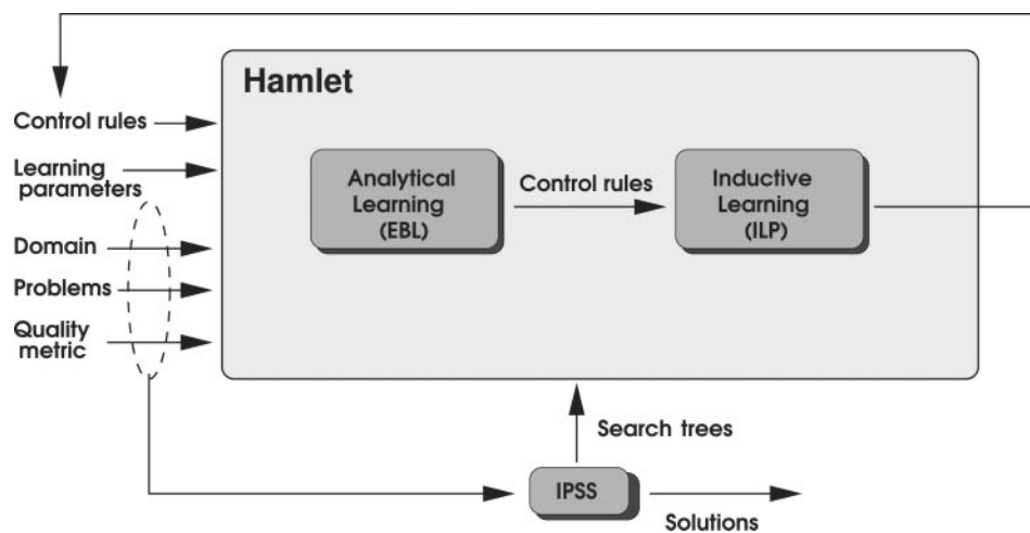
Figure 4 HAMLET high-level architecture
