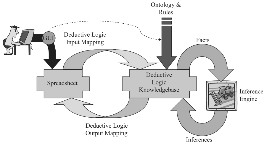
Figure 2 Deductive logic spreadsheet architecture
