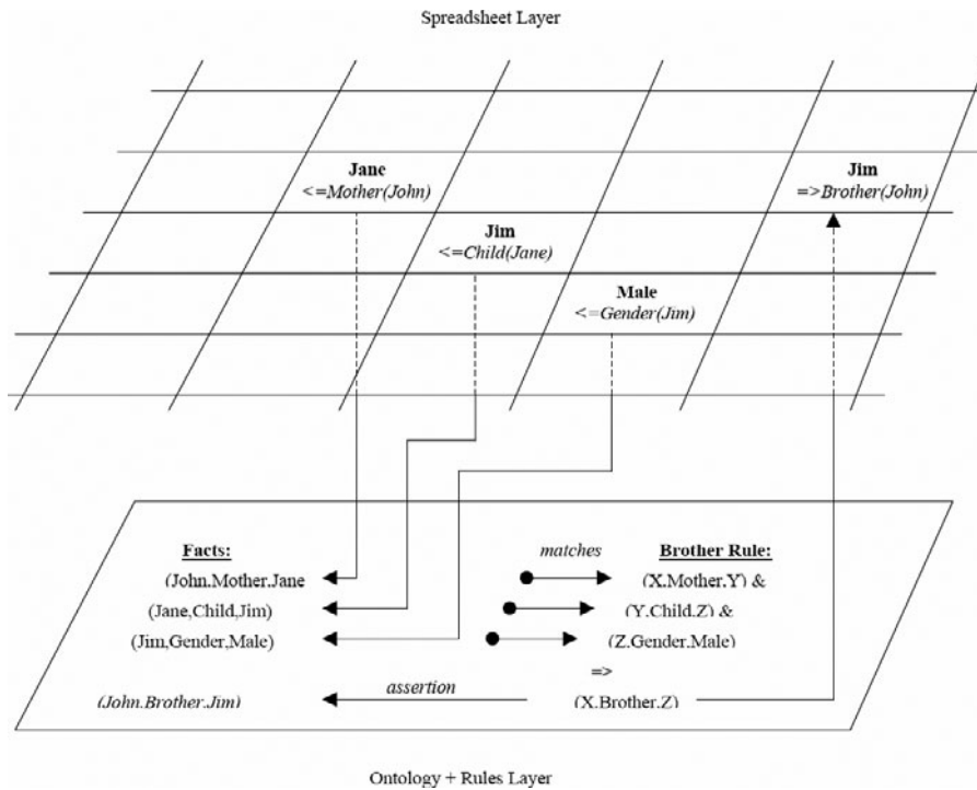
Figure 3 Mapping data between spreadsheet and knowledgebase
