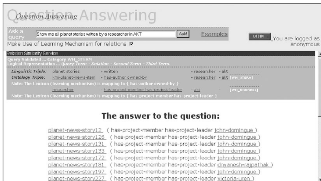
Figure 7 Aqualog interface showing at the top, the input natural language query, then intermediate triples identified by the system and finally answers. Links in the answers take the user to the original resources
