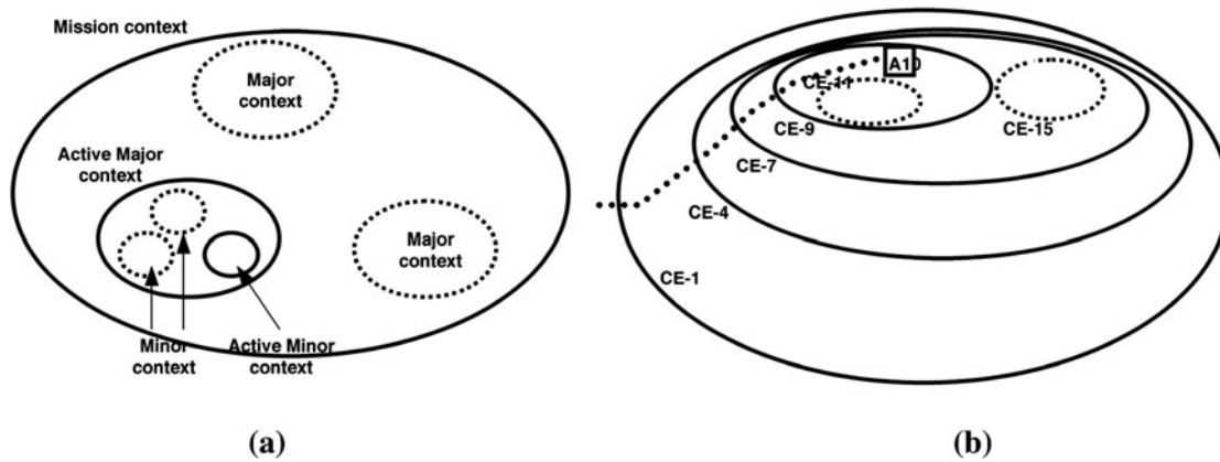
Figure 5 Operational representations of CxBR (a) and CxG (b) approaches vis-à-vis their granularity
