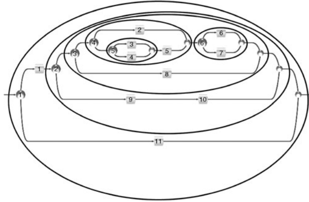
Figure 4 Context organization in CxGs
