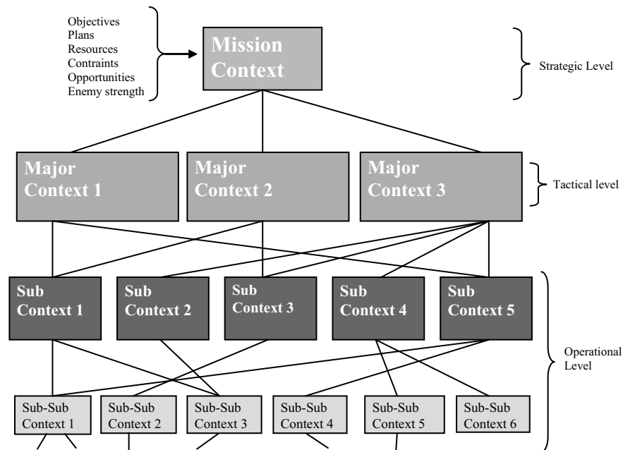
Figure 1 CxBR hierarchical organization for a particular mission
