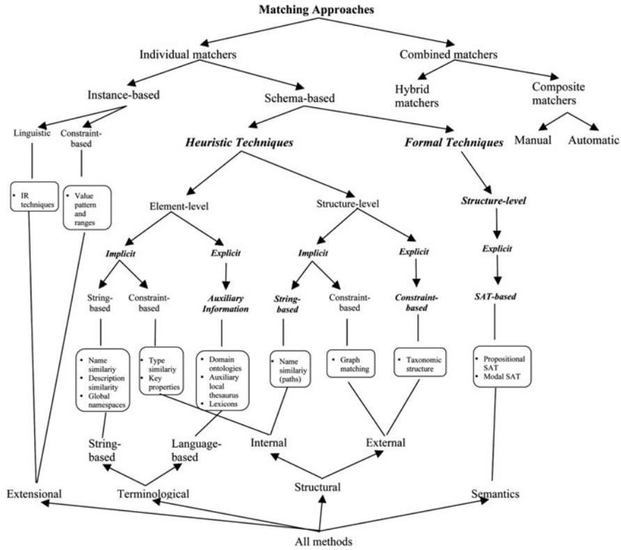
Figure 2 Classification of matching approaches
