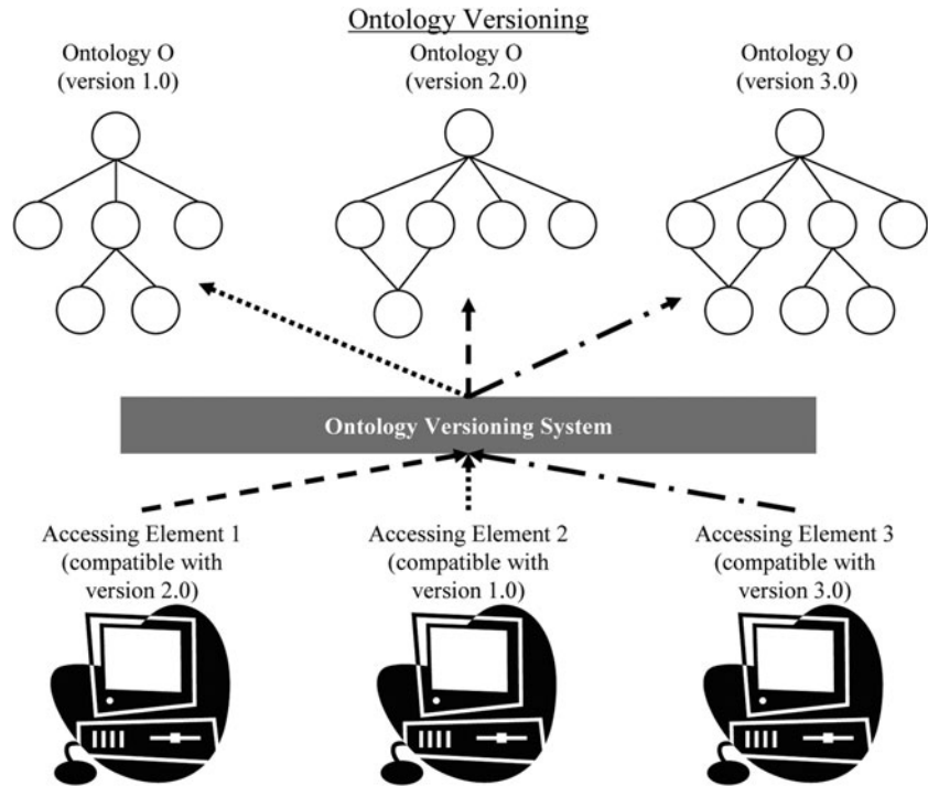
Figure 5 Ontology versioning
