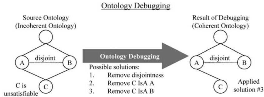
Figure 4 Ontology debugging
