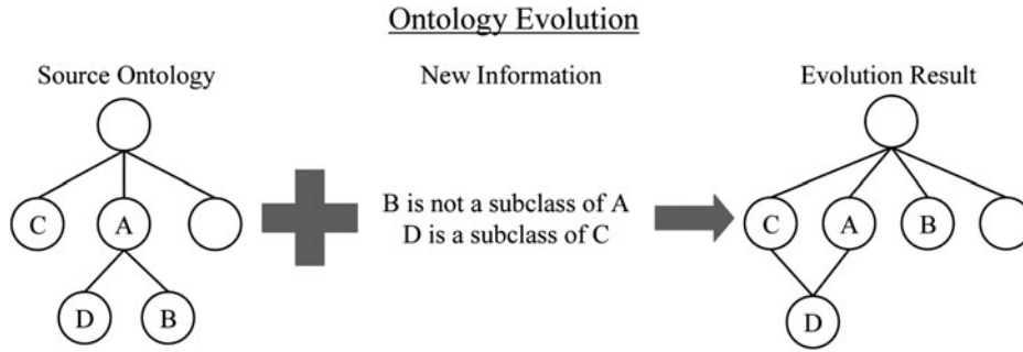
Figure 3 Ontology evolution
