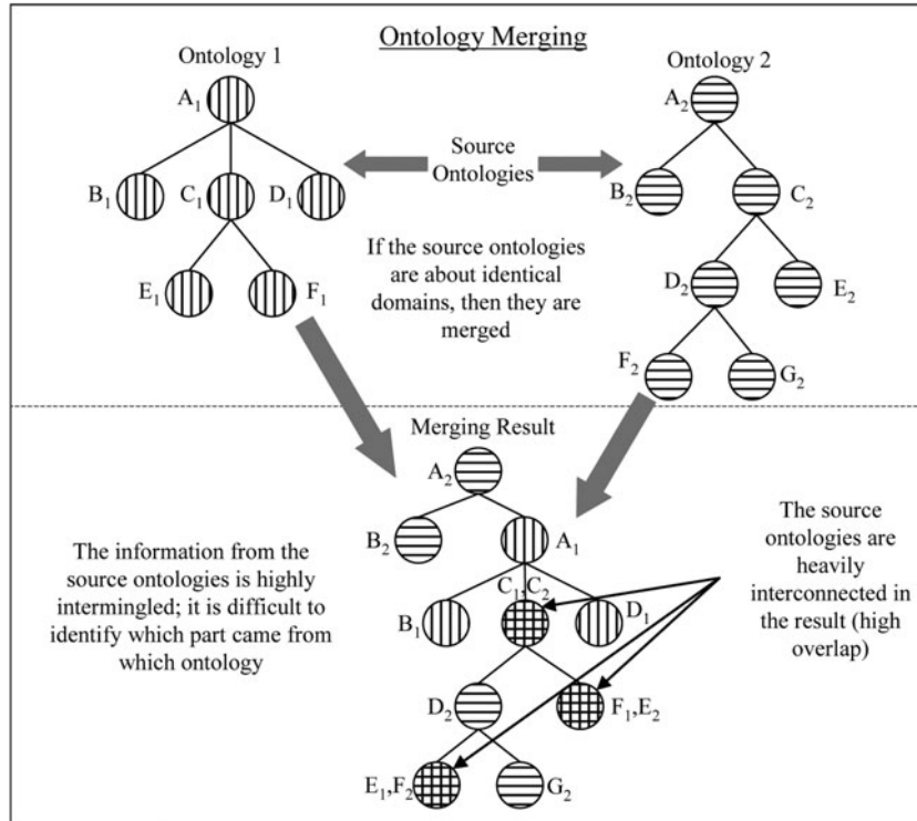
Figure 7 Ontology merging
