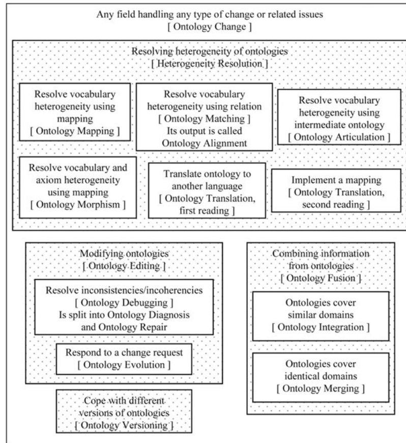
Figure 1 A classification of ontology change subfields
