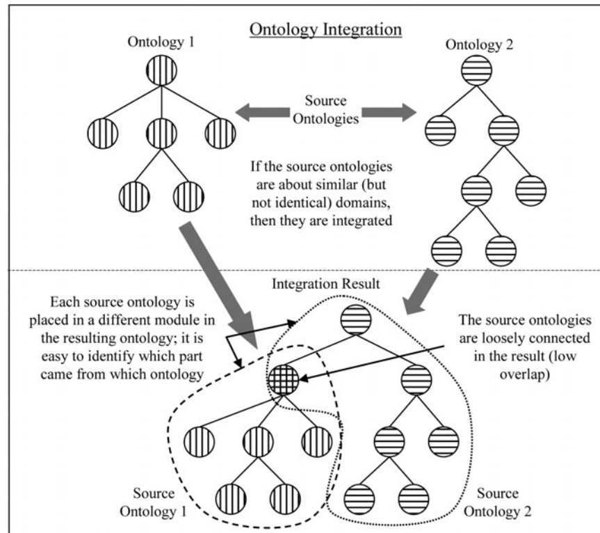
Figure 6 Ontology integration
