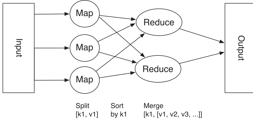
Figure 1 Map and reduce operations
