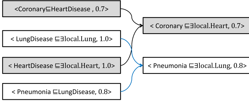
Figure 6 A joint-based partition example
