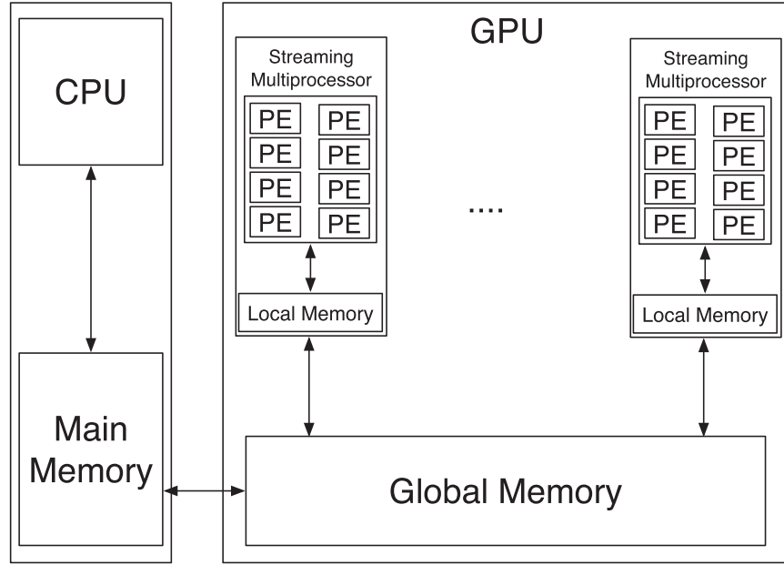
Figure 2 GPU architecture
