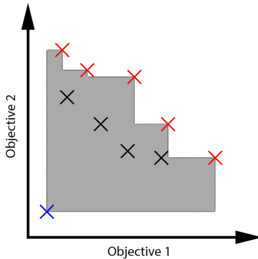
Figure 1 Solutions in red form the non-dominated set (NDS), while solutions in black are said to be dominated. The shaded area denotes the hypervolume of the NDS with respect to the reference point (shown in blue).
