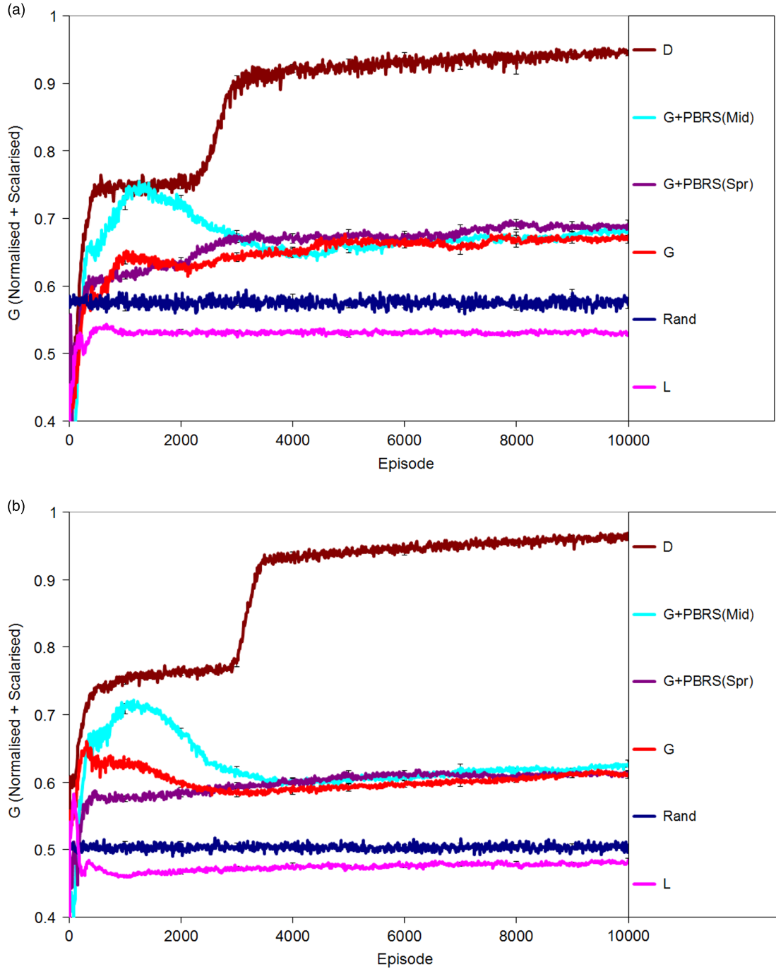
Figure 2 Average performance on normalized scalarized global reward
