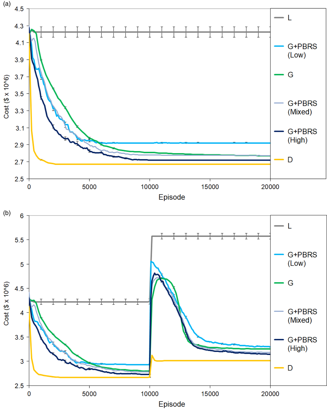
Figure 6 Learning curves for the cost objective
