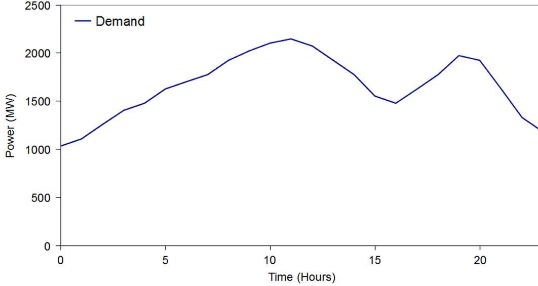
Figure 5 Twenty-four-hour power demand
