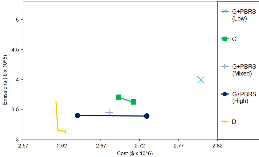
Figure 7 Best non-dominated episodes over all runs
