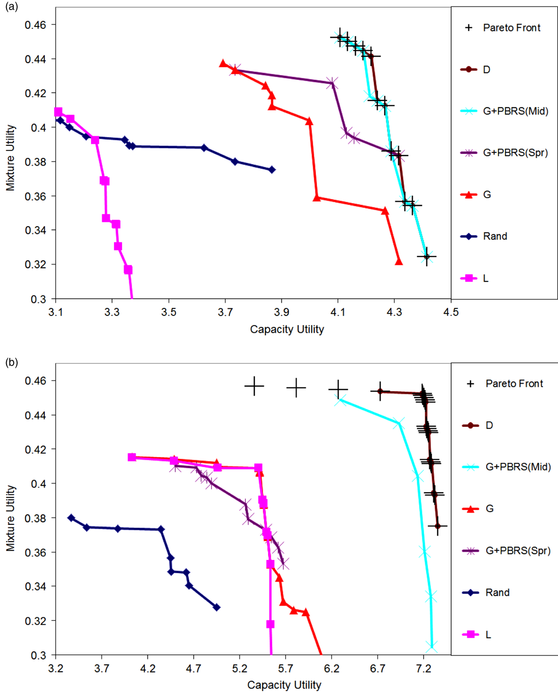
Figure 4 Best non-dominated episodes over all runs
