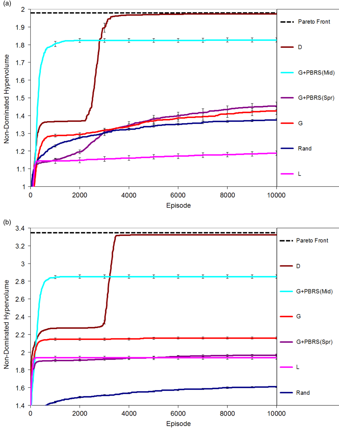
Figure 3 Average hypervolume of non-dominated solutions found
