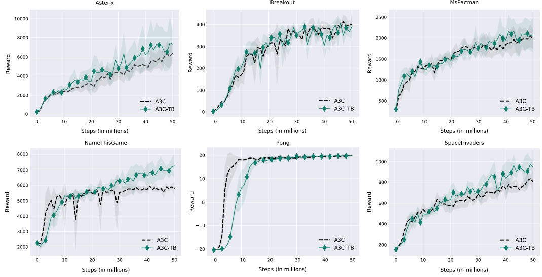
Figure 2 Performance of the baseline A3C and the TB operator variant A3C (A3C-TB). The x -axis is the total number of training steps (among all 16 actors), where each step consists of four game frames (we use frame skip of four). The y -axis is the average testing score over four trials where the shaded regions correspond to the standard deviation
