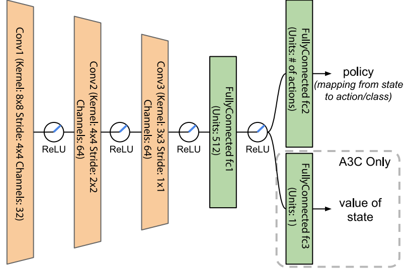
Figure 1 Network architecture for each parallel actor in the A3C agent. We follow the same architecture as in Mnih et al. (2015), where there are three convolutional layers ( conv1 , conv2 , and conv3 ), followed with two fully connected layers ( fc1 and fc2 ), and a third fully connected layer ( fc3 ) for learning the state value function as was done in Mnih et al. (2016)
