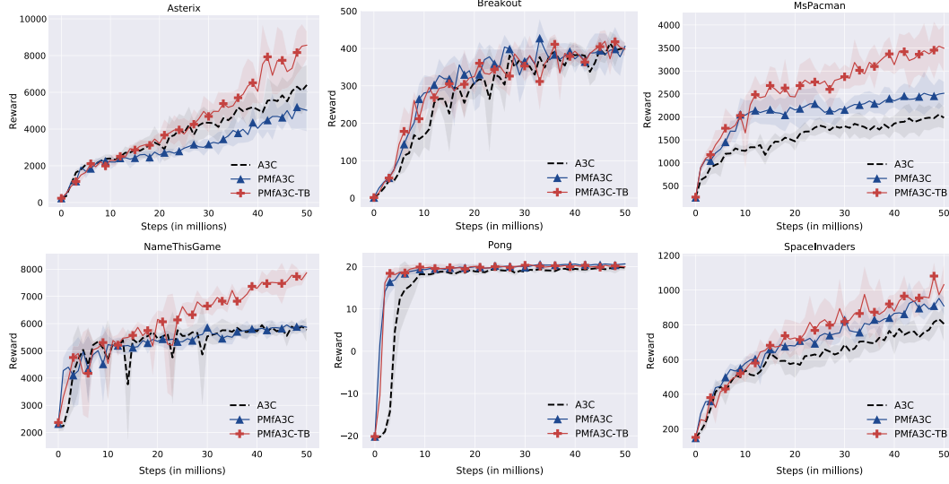
Figure 3 Performance of baseline and pre-training using A3C. The x-axis is the total number of training steps (among all 16 actors), where each step consists of four game frames (we use frame skip of four). The y-axis is the average testing score over four trials where the shaded regions correspond to the standard deviation
