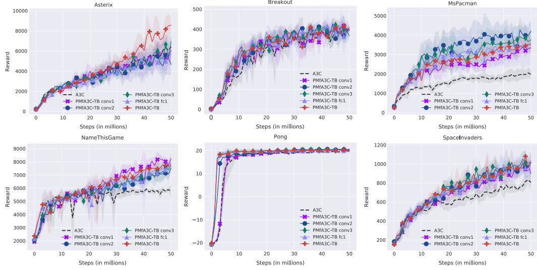
Figure 4 Performance of baseline and pre-training using A3C. The x -axis is the total number of training steps (among all 16 actors), where each step consists of four game frames (we use frame skip of four). The y -axis is the average testing score over four trials where the shaded regions correspond to the standard deviation
