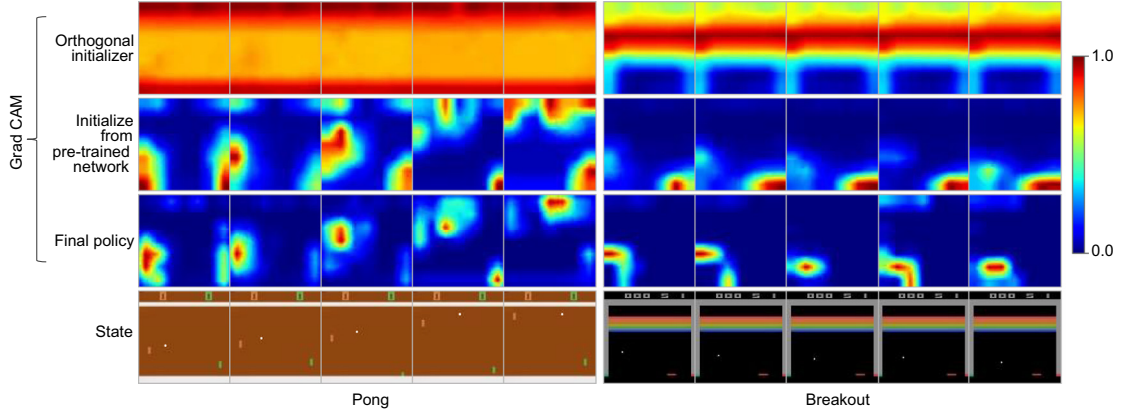
Figure 5 (Color online) Gradient-weighted Class Activation Mapping visualization for Pong and Breakout. Top row: random initialization; second row: pre-trained model; third row: final learned RL policy; bottom row: the original game image
