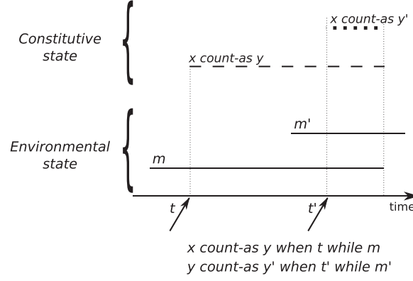
Figure 3 Example of constitutive state changes along time. At some moment, while a state m holds, an event t happens (cf. the first arrow in the bottom of the picture). By the constitutive rule x \text{ count-as } y \text{ when } t \text{ while } m ( \langle x, y, t, m \rangle \in C ), such conditions lead the environmental element x to count as y in the constitutive state (cf. the dashed line). Then, the event t' occurs while the state m' holds. By the constitutive rule y \text{ count-as } y' when t' while m' , the element that counts as y (i.e. x ) counts also as y' (cf. the dotted horizontal line). When the state m ceases to hold, the conditions to x count as y also cease to hold, and as x is no longer counting as y , it also ceases to count y' . For example, if x = \text{bob} , y = \text{bidder} , and y' = \text{auction\_participant} , s.t. \text{bob} \in A_X and \{\text{bidder}, \text{auction\_participant}\} \subseteq A_F , then \text{bob} counts as (i) \text{bidder} from t and (ii) \text{auction\_participant} from t'
