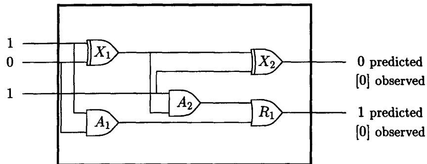
Figure 5 Full adder.
