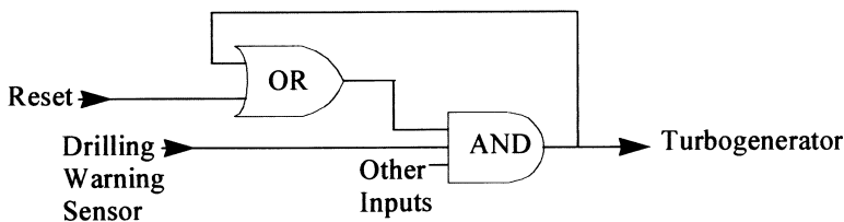
Figure 4 Logic diagram of latched reset
