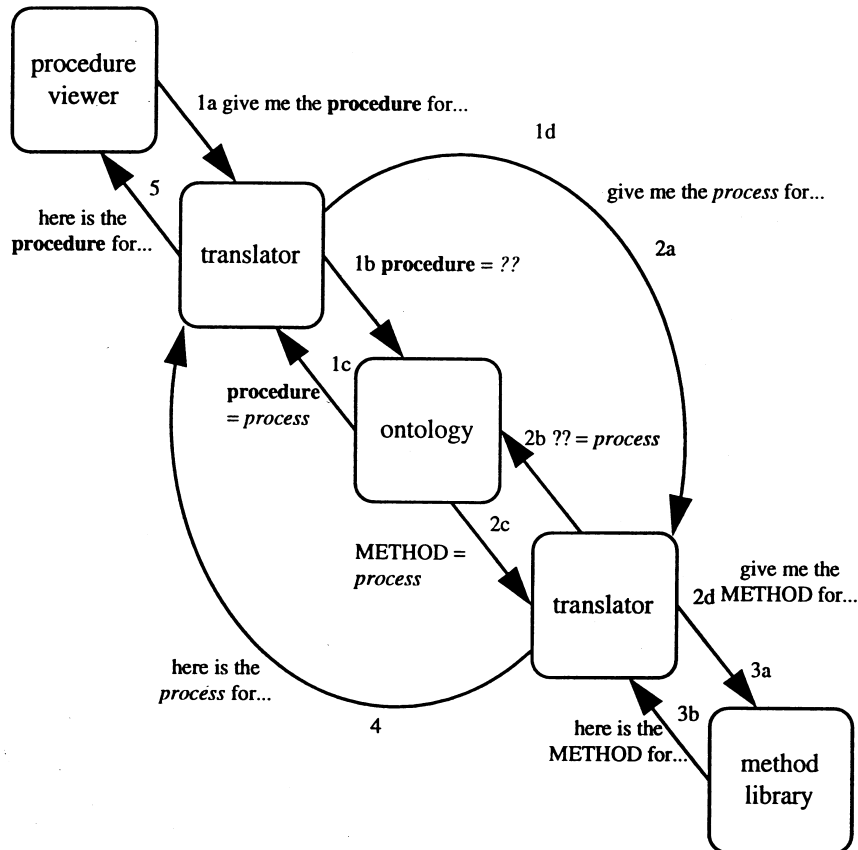
Figure 2 Interchange format example. This illustrates the use of an ontology as an interchange format to integrate different software tools. The term procedure , used by one tool is translated into the term, method used by the other via the ontology, whose term for the same underlying concept is process .
