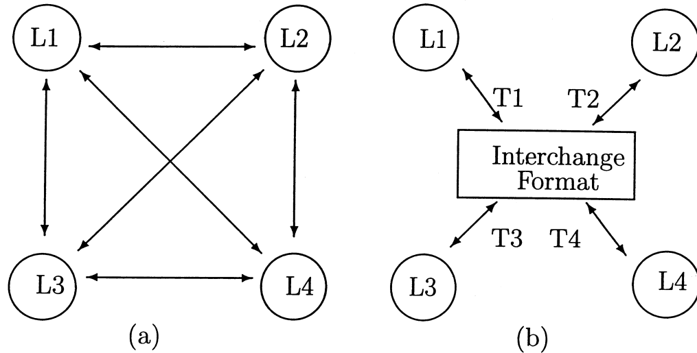
Figure 3 Interchange format. To translate from language L_i to L_j and vice versa , a translator is required between L_i and the interchange format and another between the interchange format and L_j . Thus, given n languages, only O(n) translators are required, not O(n^2) .
