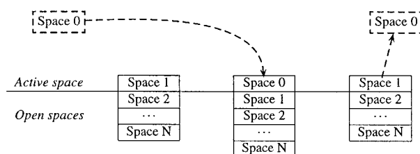
Figure 2 Examples of stack movements. Space 0 becomes the new active space. Then it is popped and Space 1 becomes active again.
