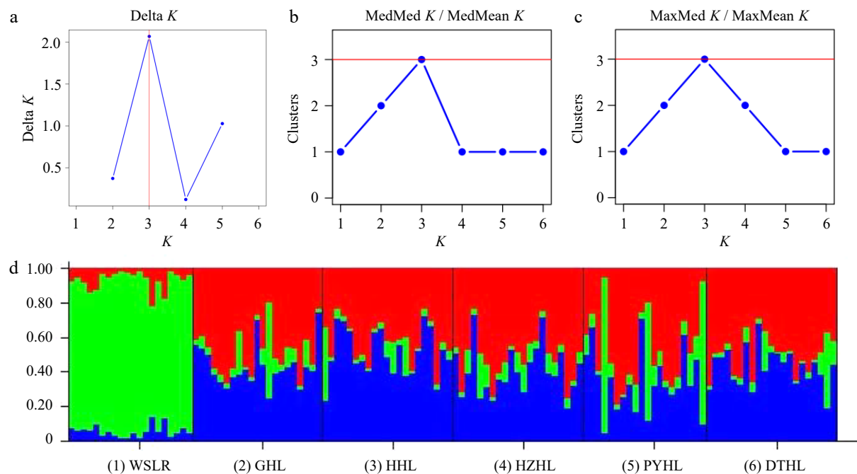
Fig. 4 Ancestral lineage analysis of six yellow catfish populations. (a) Delta K , (b) MedMed K / MedMean K , and (c) MaxMed K / MaxMean K plots indicating the best number of clusters ( K ) of the STRUCTURE analysis. (d) Cluster assignment from STRUCTURE averaged over six replicated runs for K = 3 . Colors represent different clusters.
