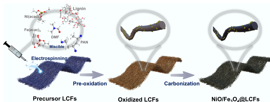
Fig. 1 Schematic diagram of the synthesis of NiO/Fe 3 O 4 @LCFs.
