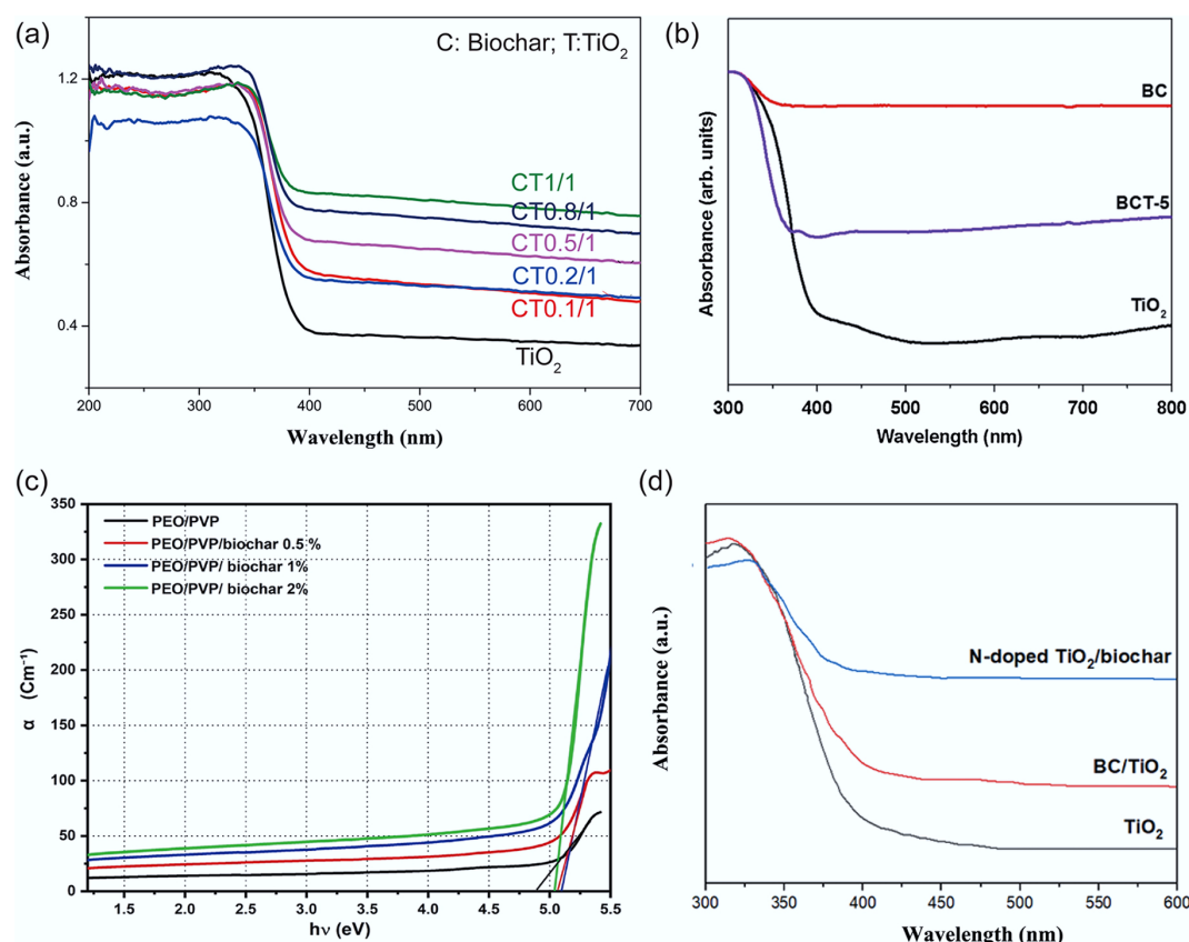
Fig. 8 (a) UV-vis diffuse reflectance spectra of \text{TiO}_2 and biochar/ \text{TiO}_2 composites [93] . (b) UV-vis diffuse reflectance spectra of biochar, \text{TiO}_2 , and biochar/ \text{TiO}_2 composites [94] . (c) Absorption coefficient ( \alpha ) vs photon energy ( h\nu ) of PEO/PVP/biochar composite [95] . (d) UV-vis spectra of \text{TiO}_2 , BC/ \text{TiO}_2 , and N-doped \text{TiO}_2 /biochar powder [96] .
