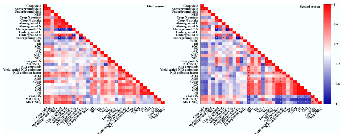
Fig. 5 Relationships between crop yields, crop nutrient contents, soil physicochemical and microbial properties, inorganic N supply and immobilization rates, and soil \text{N}_2\text{O} emissions. WHC, water holding capacity; SOC, soil organic C; TN, total N; GNM, gross N mineralization; GN, gross nitrification; GAI, gross \text{NH}_4^+ immobilization; GNI, gross \text{NO}_3^- immobilization; GI, gross immobilization; \text{MRT NH}_4^+ , mean residence time of \text{NH}_4^+ ; \text{MRT NO}_3^- , mean residence time of \text{NO}_3^- . * indicates p < 0.05 .
