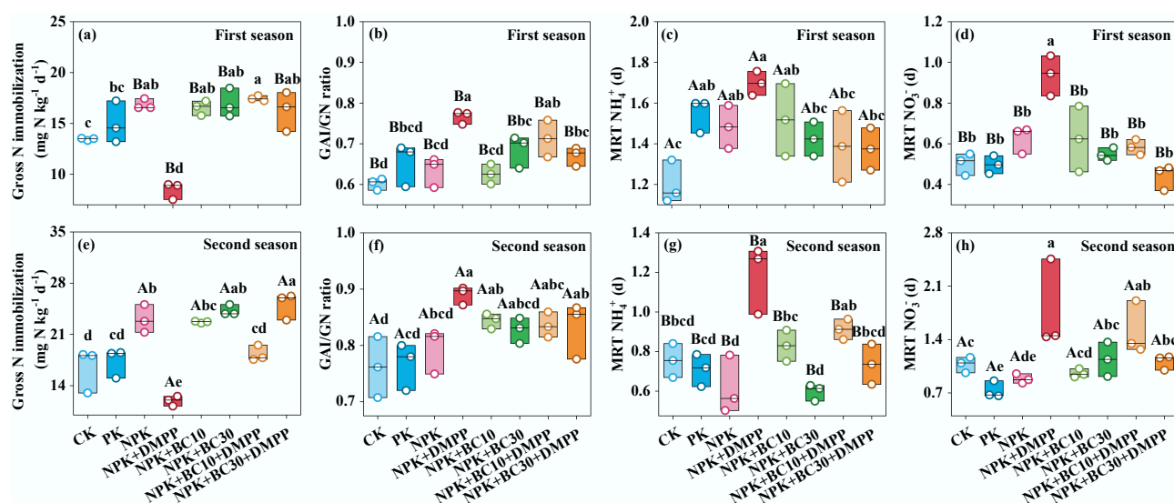
Fig. 4 Changes in (a), (e) gross N immobilization, (b), (f) gross \text{NH}_4^+ immobilization/gross nitrification (GAI/GN) ratio, (c), (g) mean residence time of \text{NH}_4^+ ( \text{MRT NH}_4^+ ), and (d), (h) mean residence time of \text{NO}_3^- ( \text{MRT NO}_3^- ) after fertilizer application during the first and second seasons. Different lowercase and uppercase letters indicate significant differences between fertilization treatments and growing seasons, respectively. The absence of letters indicates no significant differences. The values represent the average \pm standard deviation ( n = 3 ).
