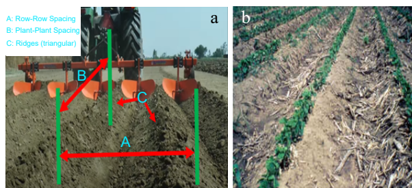
Fig. 10 Ridge-planting technique for cotton: (a) A five-row ridger making fresh ridges in a cotton field, with illustrated general planting geometry. (b) Ridged field cultivated with new crops while the previous year growth/crop residue remains in the furrow, helping with erosion control, typically, 30%–50% nonuniformly distributed residue may be found in row-crop rotated ridge-sowing fields [77] .
