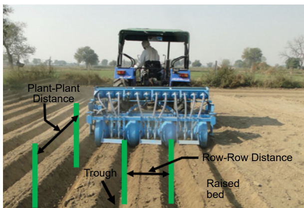
Fig. 8 An image showing a multi-crop raised seedbed planter operating on a field with illustrated bed configuration parameters. The machine first creates the raised trapezoidal seedbeds and plants the seeds in its trail. (Image adapted from Kumar et al. [73] ).
