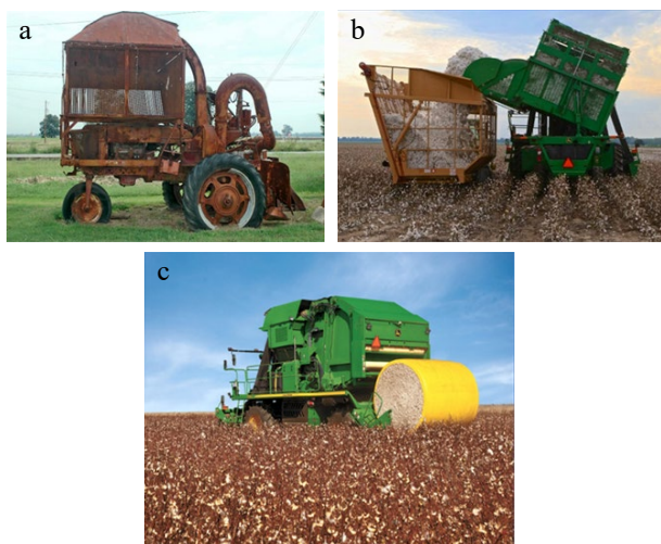
Fig. 6 Evolution of mechanized cotton harvesting. (a) A second generation commercially successful cotton picker M produced in the 1940s. (b) A boll buggy receiving seed cotton from a cotton picker, an approach that required multiple equipment types and is labor intensive. (c) A 7760 JD cotton harvester with onboard module building feature, requiring no extra human labor and expensive equipment and tractors to build cotton modules. (Sources: (a) Mississippi State University Extension, (b) West Tennessee Historical Society, and (c) John Deere, Inc.).
